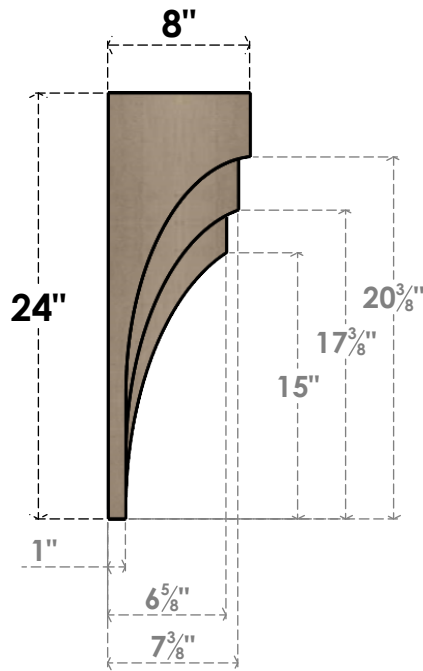
SIDE PROFILE
